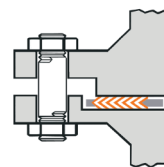
Type HX-R-IR As HX-R but with inner ring
