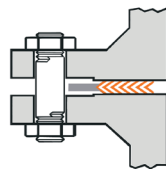
Type SG Gasket with guide ring to act as compression stop
